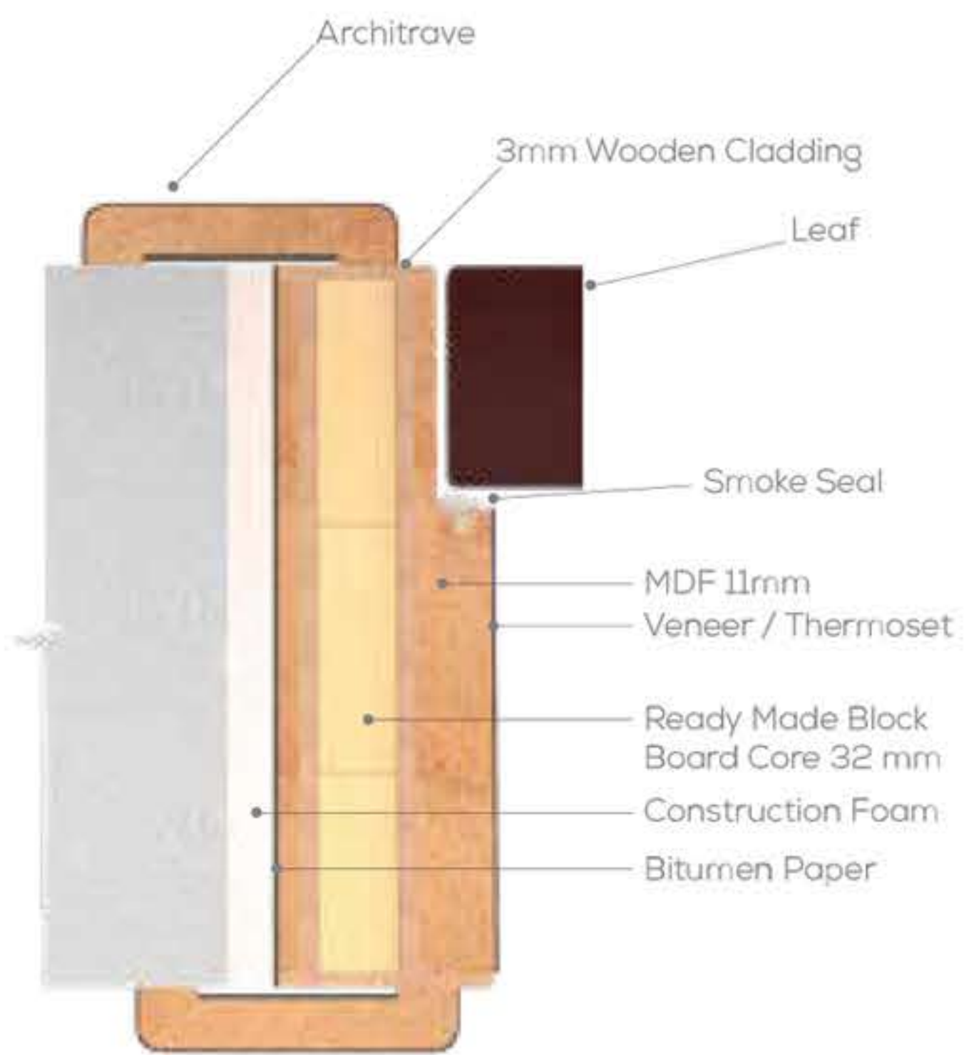
VENEERED JAMB FRAME (VENEERED, THERMOSET & PAINTED)
