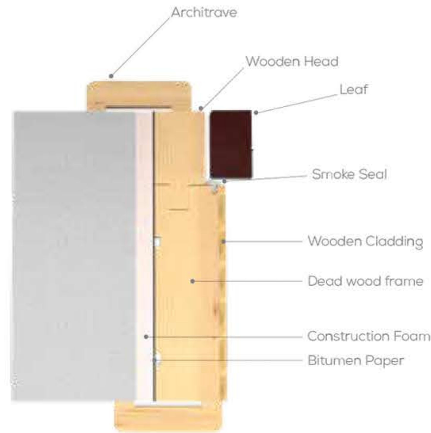
ENGINEERED JAMB FRAME (WITH CLADDING)
