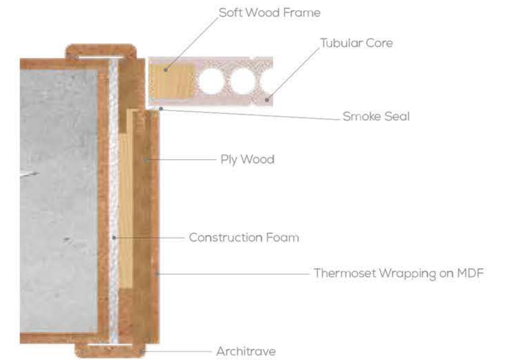
PLY WOOD JAMB FRAME
