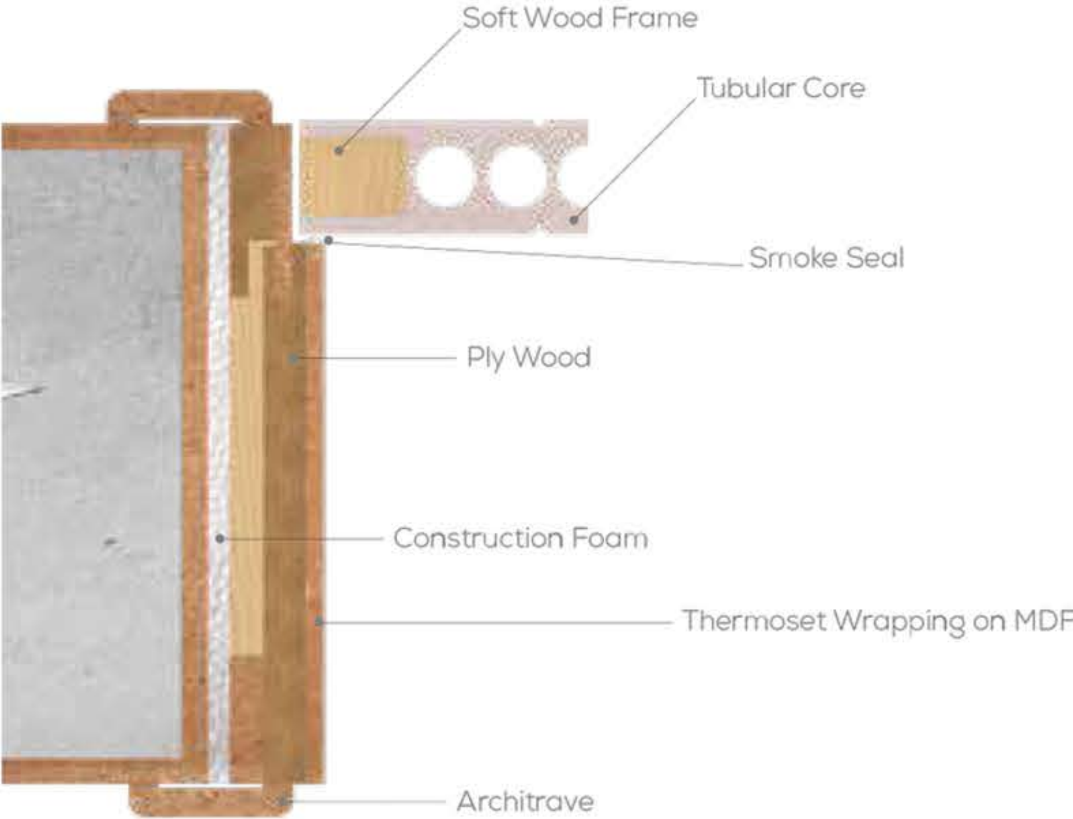
PLY WOOD JAMB FRAME
