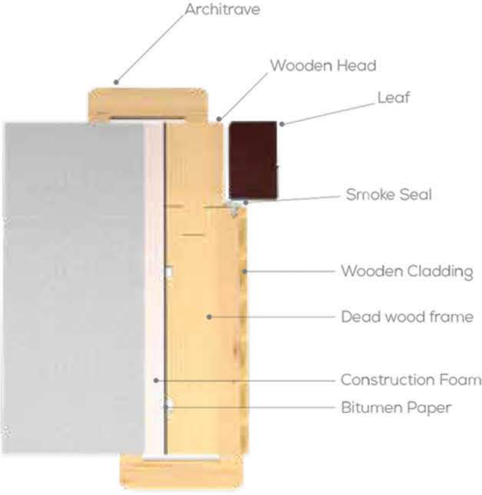
ENGINEERED JAMB FRAME (WITH CLADDING)
